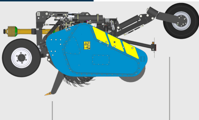
Ripper tines equipped with hydraulic safety devices
